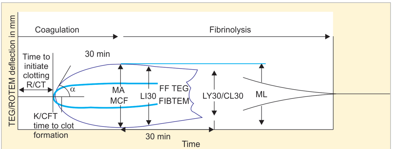
Figs 1 A to C: Schematic illustration of (A) TEG mechanism and machine, (B) ROTEM mechanism and machine, and (C) a representative TEG/ROTEM tracing showing the relationship between the qualitative tracing and the quantitative parameters. Courtesy: Haemonetics Corporation and TEM Systems, Inc.
